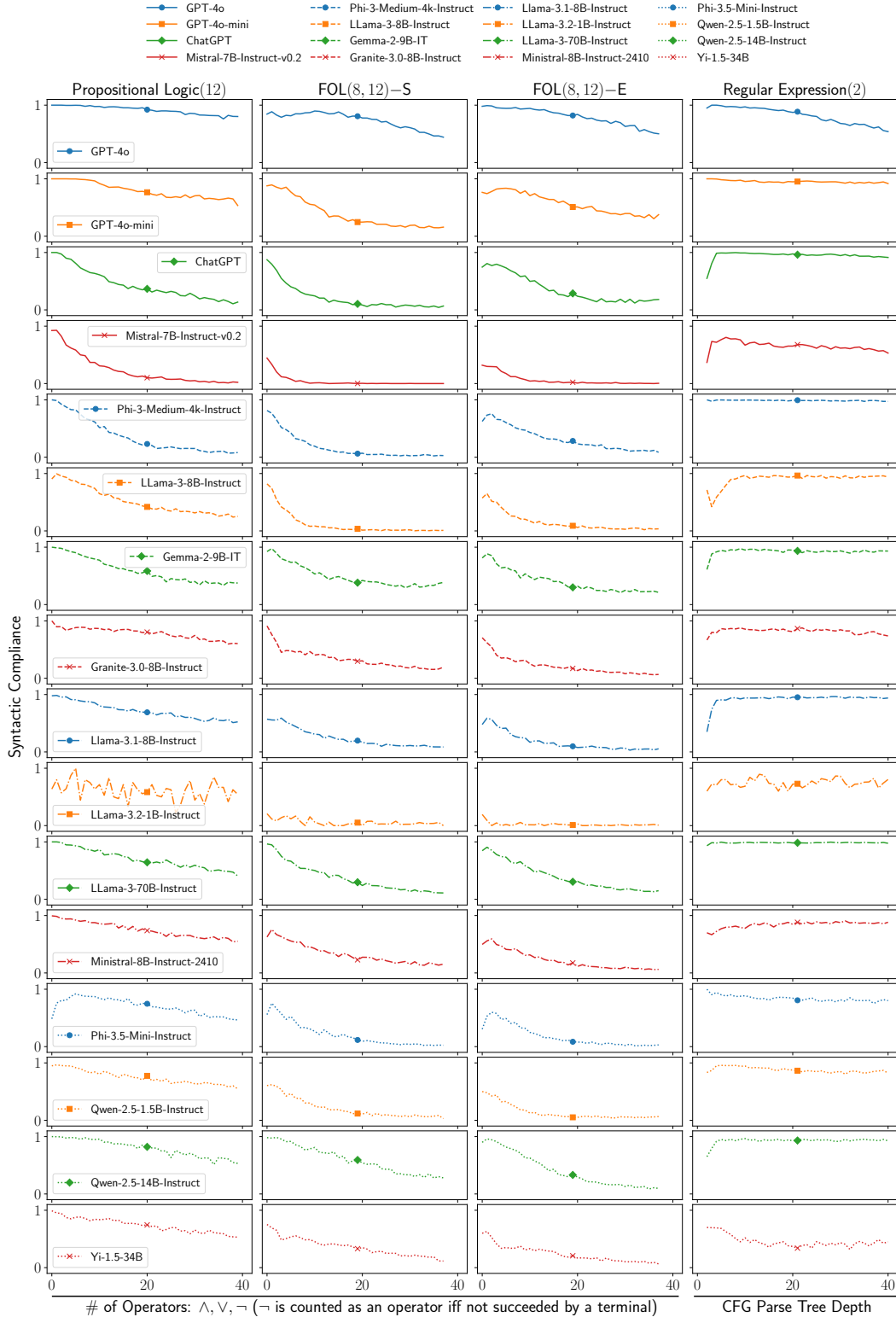
Figure 18: Syntactic compliance (§A1) of all models on the \forall\text{uto}\exists\forall\wedge\text{L} datasets.
