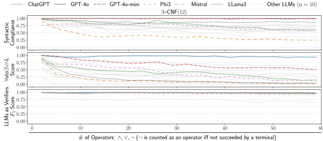
Figure 7: Zero-shot Pass@1 results (avg. over 10 batches, higher values better) for 3-CNF from using \forall\text{uto}\exists\forall\wedge\text{L} to assess LLMs w.r.t. §A1, §A2, §A3 (Sec. 3.3.1) on the packaged datasets. The x-axis is the # of operators.
