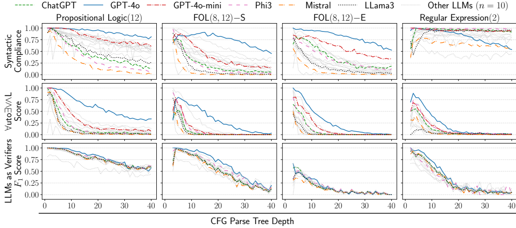
Figure 11: Zero-shot Pass@1 results (avg. over 10 batches, higher values better) from using \forall\text{Auto}\exists\forall\text{L} to assess LLMs w.r.t. §A1, §A2, §A3 (Sec. 3.3.1) on the packaged datasets. The x-axis is the depth of the CFG tree to produce the formula.
